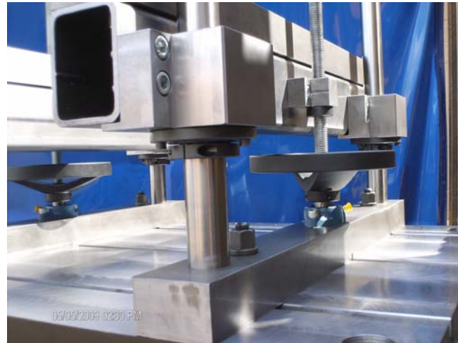
X-Y-Z positioner unit with 7-pillar guide for the mounting of a driving unit
