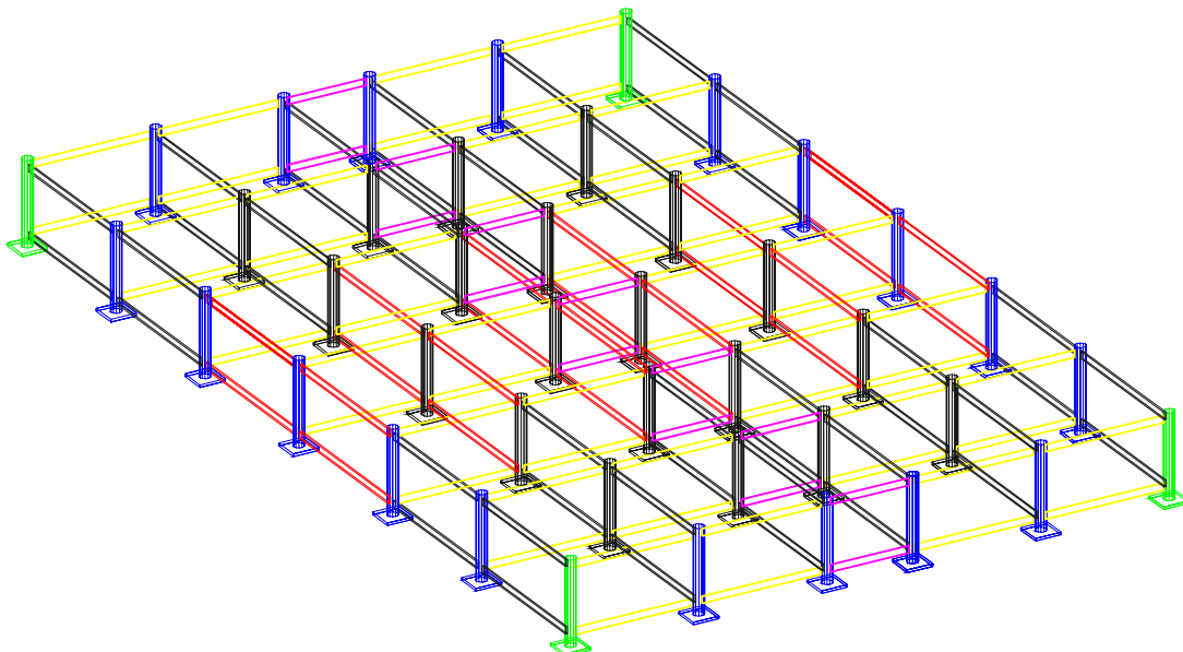
anchor frame construction 3D view
